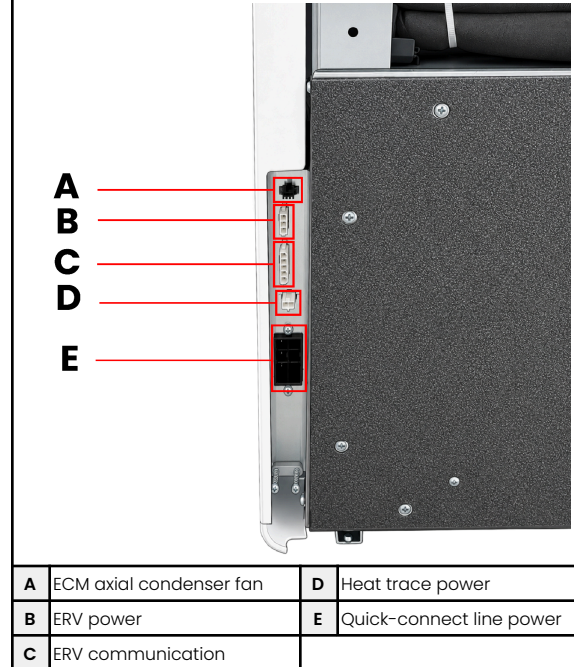
Figure 6. Gen 3 Accessory connection locations
