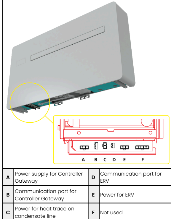
Figure 5. Gen 2 Accessory connection locations
