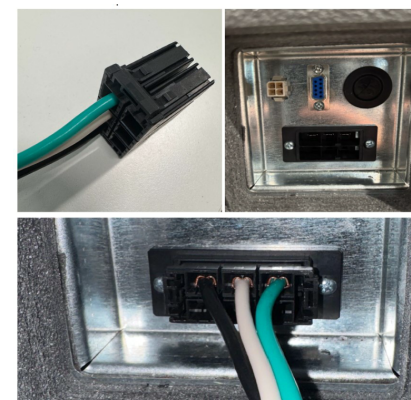
Figure 2. Quick Connect on the Vertical Stack
