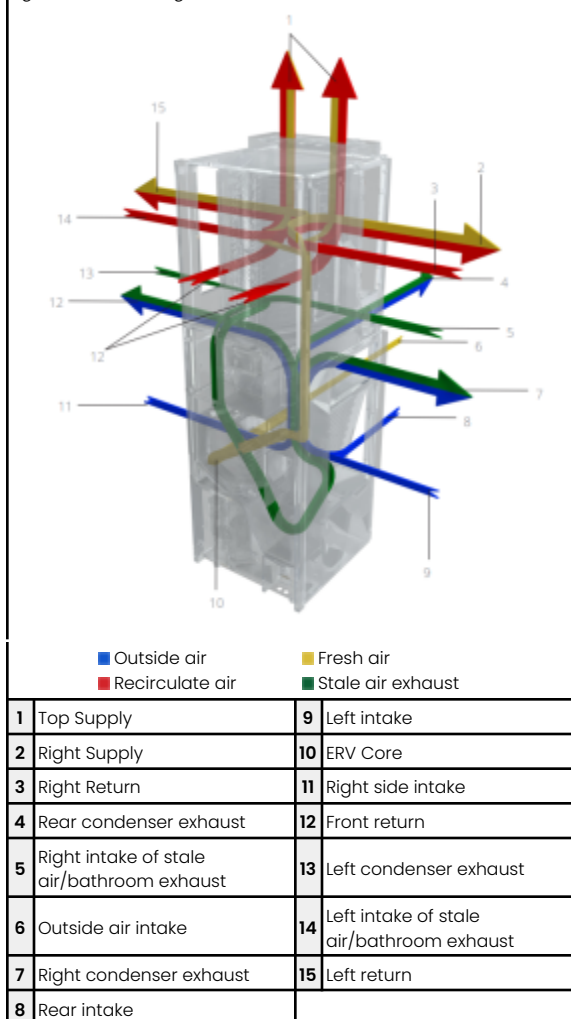
Figure 3. Airflow diagram
