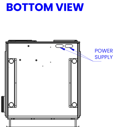
Figure 16. AIO™ Vertical Stack XL dimensions (bottom view)
