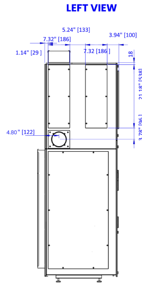
Figure 15. AIO™ Vertical Stack XL dimensions (left view)
