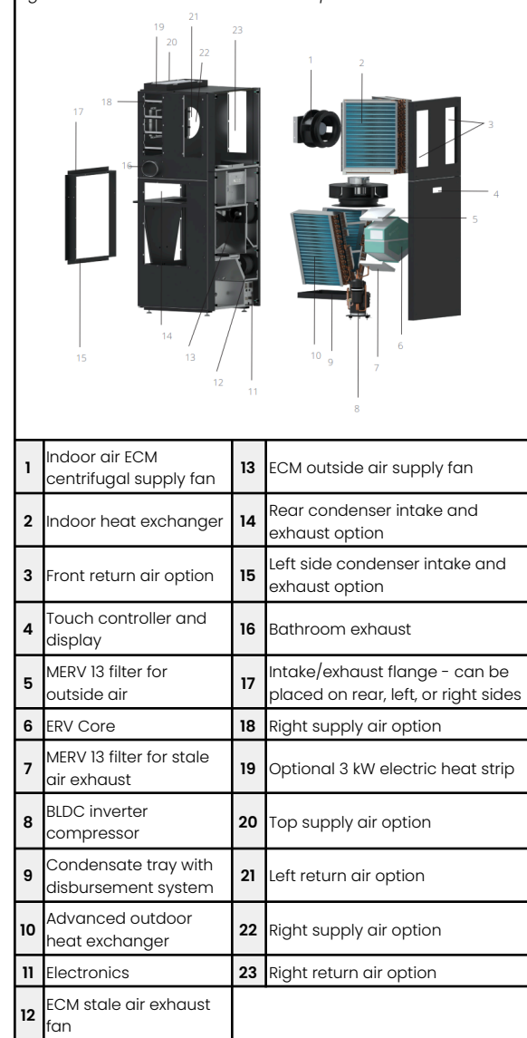
Figure 2. Vertical Stack XL with ERV components and structure
