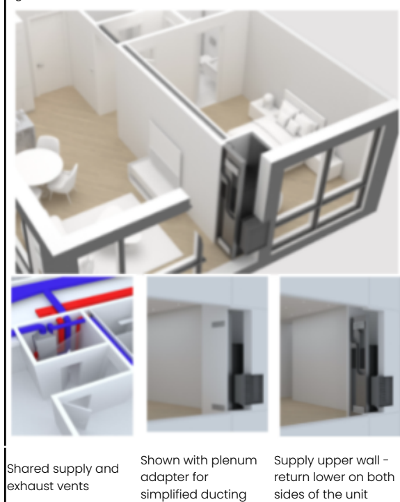
Figure 9. Installation
