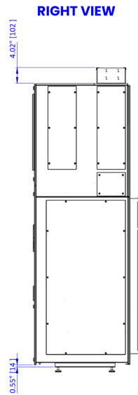
Figure 13. AIO™ Vertical Stack XL dimensions (right view)
