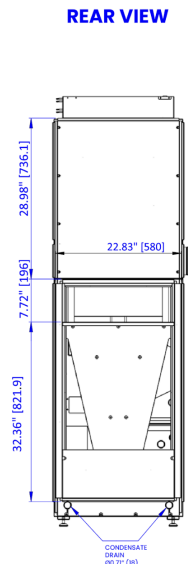
Figure 14. AIO™ Vertical Stack XL dimensions (rear view)
