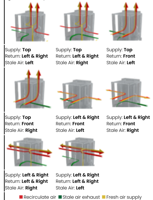
Figure 4. Fan coil part
