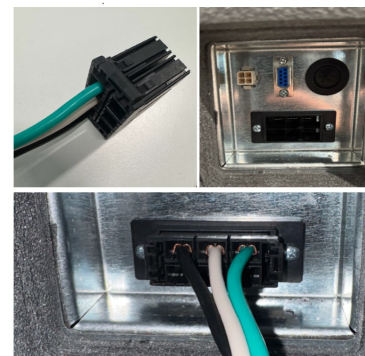
Figure 2. Connecting on the vertical stack
