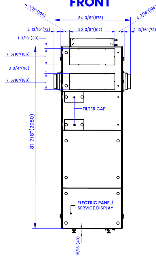
Figure 25. Front view
