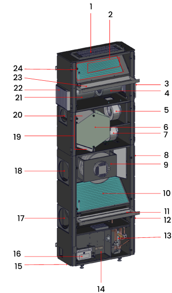
Figure 2. AIO™ Vertical Stack with ERV (R32) components and structure
