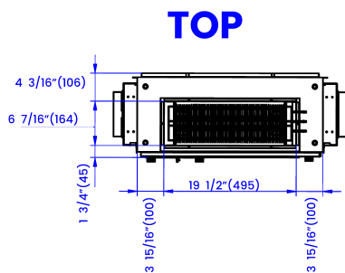
Figure 23. Top view
