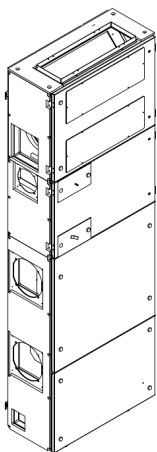
Figure 22. Vertical Stack Dimensions
