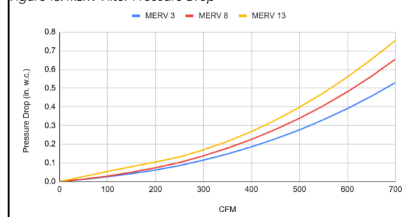
Figure 18. MERV Filter Pressure Drop
