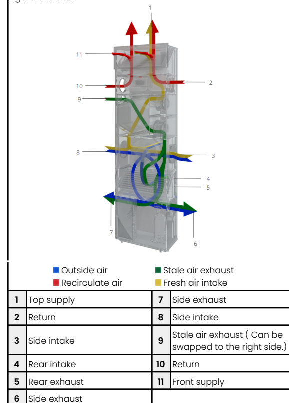
Figure 3. Airflow
