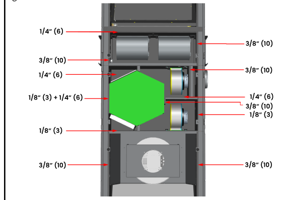
Figure 19. Insulation Thickness
