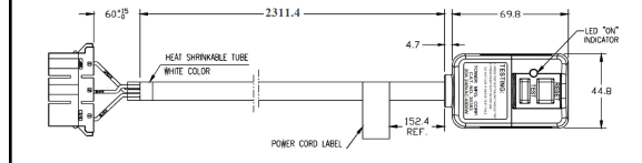
Figure 4. Cord detail
