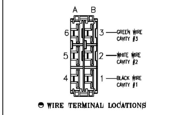
Figure 6. Wire Terminal Locations
