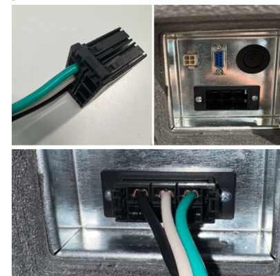
Figure 3. Quick Connect on the Vertical Stack
