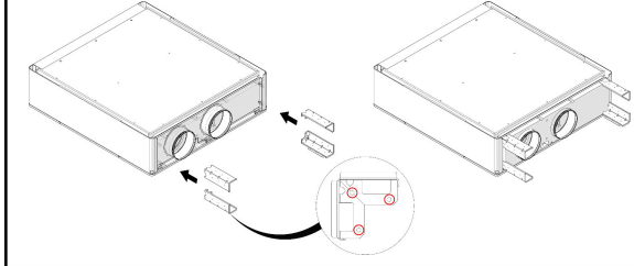
Figure 1. Installing the four brackets
